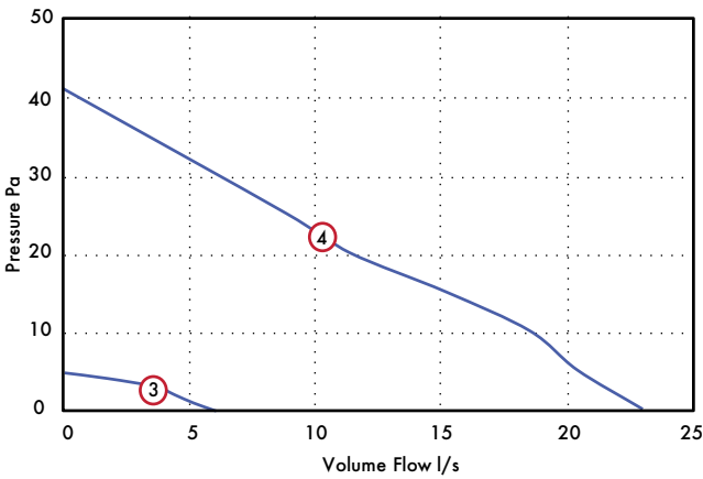
Open Grille
